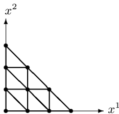
Figure 5: Additive preferences over three public goods.
